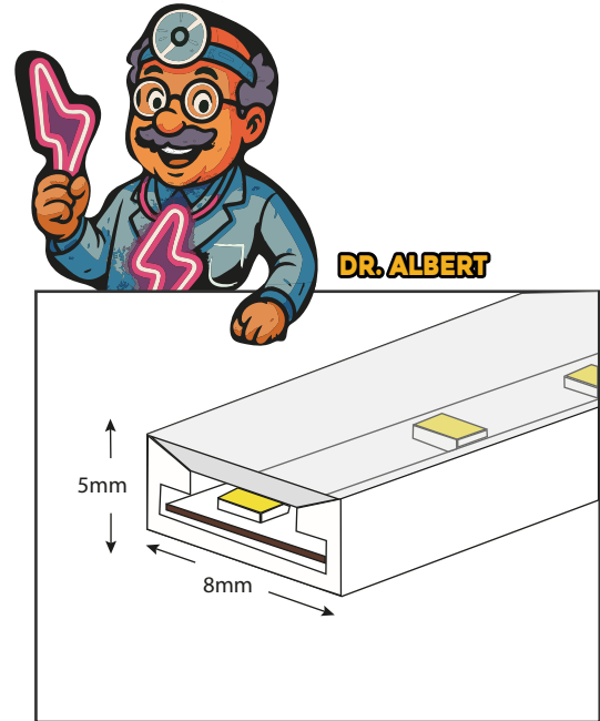
Neon LED Technical Drawing
