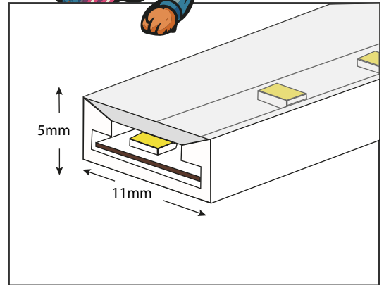
Neon LED Technical Drawing
