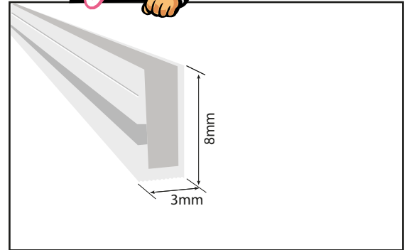
Neon LED Technical Drawing
